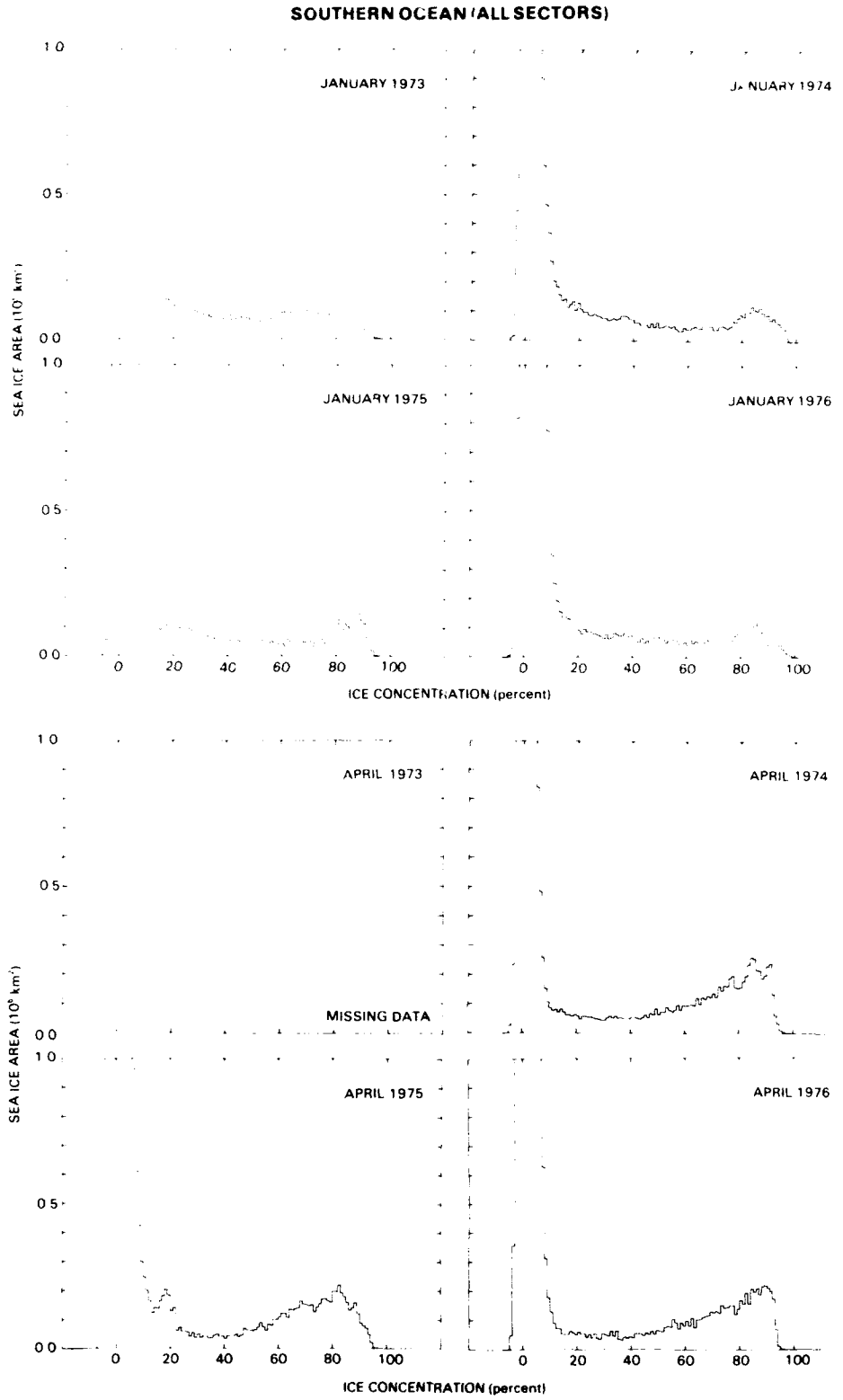
Figure C-2. Year-to-year comparison of areal distribution of percentage ice concentration in all sectors for January and April.
