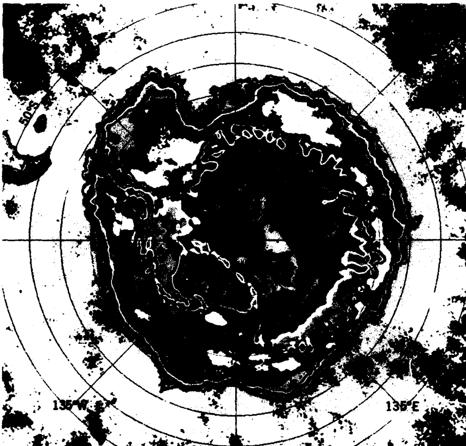
Figure 3-9b. Mean monthly brightness temperatures for June 1975 and 1976.
