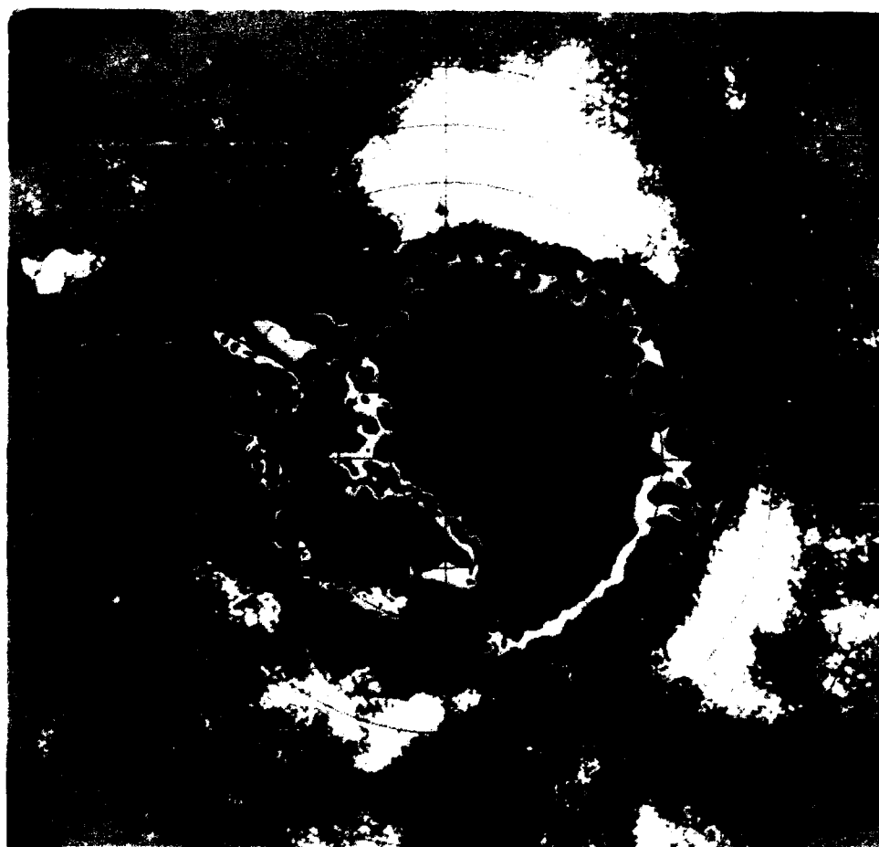
Figure 3-5a. Mean monthly brightness temperatures for February 1973 and 1974.
