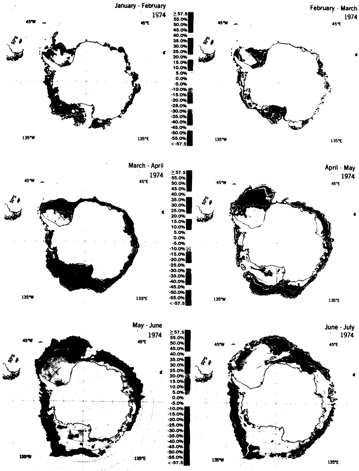
Figure 5-24a. Sea ice concentration monthly change maps for January-February 1974 through June-July 1974.
