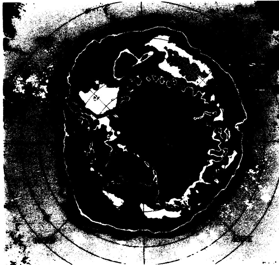
Figure 3-20. Four-year average of mean monthly brightness temperatures for September and October, 1973-1976.
