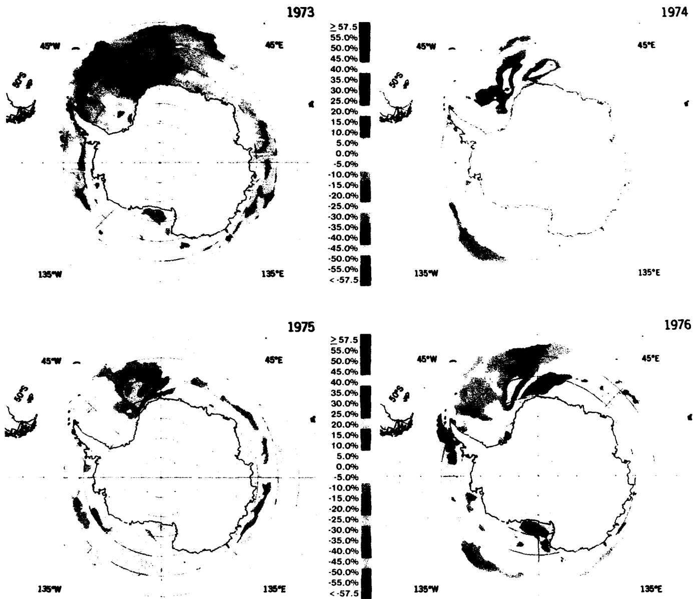
Figure 5-42. Deviations of annual mean sea ice concentrations from 4-year average of annual means.
