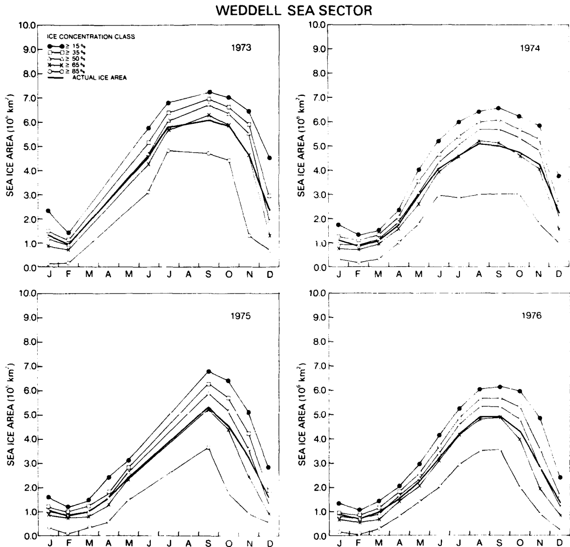
Figure 5-14. Yearly cycle of the ocean area covered by sea ice with concentration \geq 15 (ice extent), \geq 35 , \geq 50 , \geq 65 , and \geq 85 percent and yearly cycle of the actual ice area, for the Weddell Sea sector in 1973, 1974, 1975, and 1976. The actual ice area is the total ocean surface covered by sea ice, excluding all open leads and polynyas within the ice pack.
