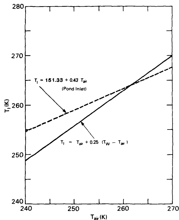
Figure 3-24. Estimated snow/ice interface temperature used to derive sea ice concentration compared with a curve fitted to Pond Inlet temperature data (Ramseier, private communication).
