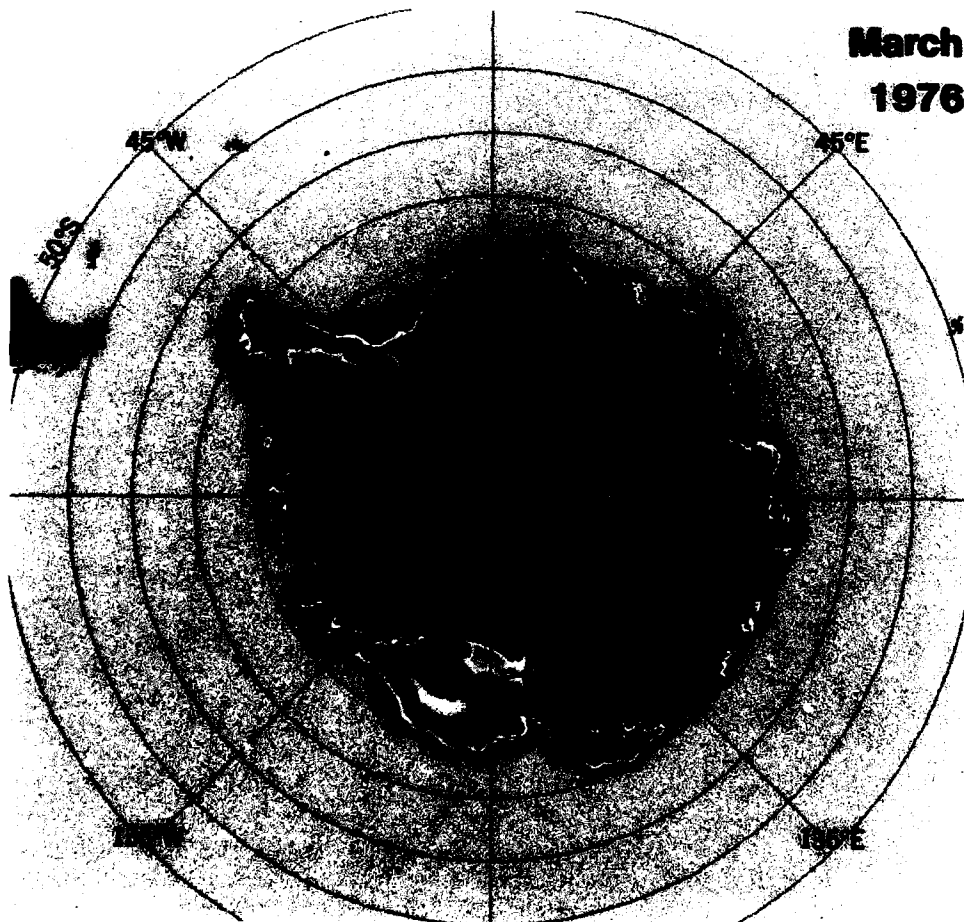
Figure 5-3b. Mean monthly sea ice concentrations for March 1975 and 1976.
