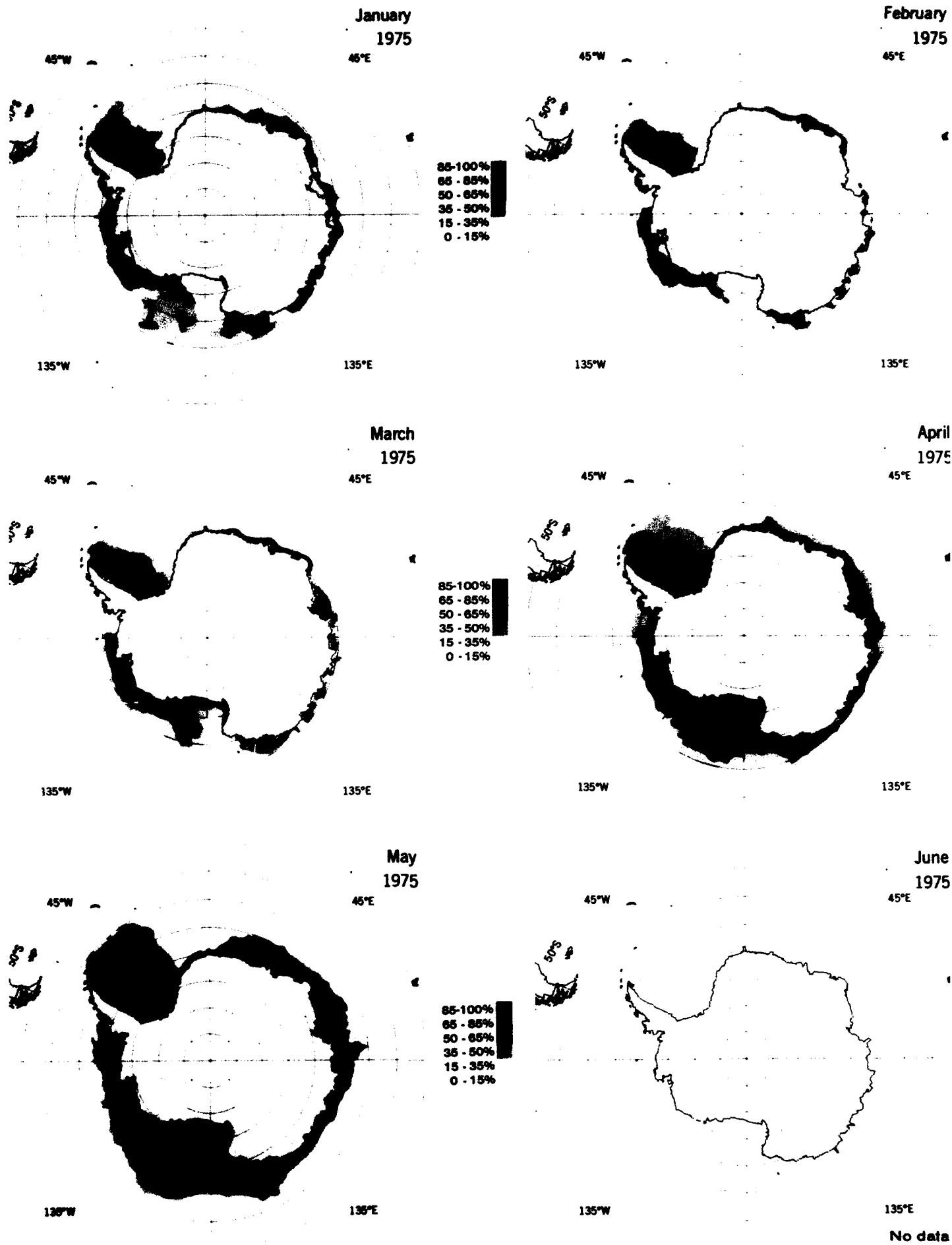
Figure B-3a. Mean monthly ice concentrations for January through June 1975.
