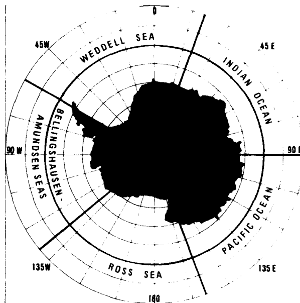
Figure 2-3. Sectors of the southern ocean used for analysis of observed sea ice cover.
