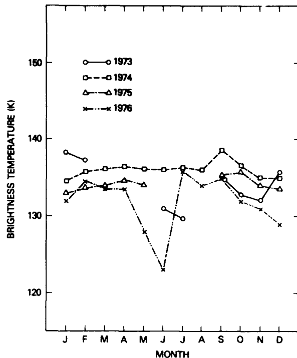
Figure A-3. Mean recorded brightness temperature of the ocean between 55^\circ\text{S} and 65^\circ\text{S} , plotted for each month, 1973 through 1976, before correction for calibration shifts.
