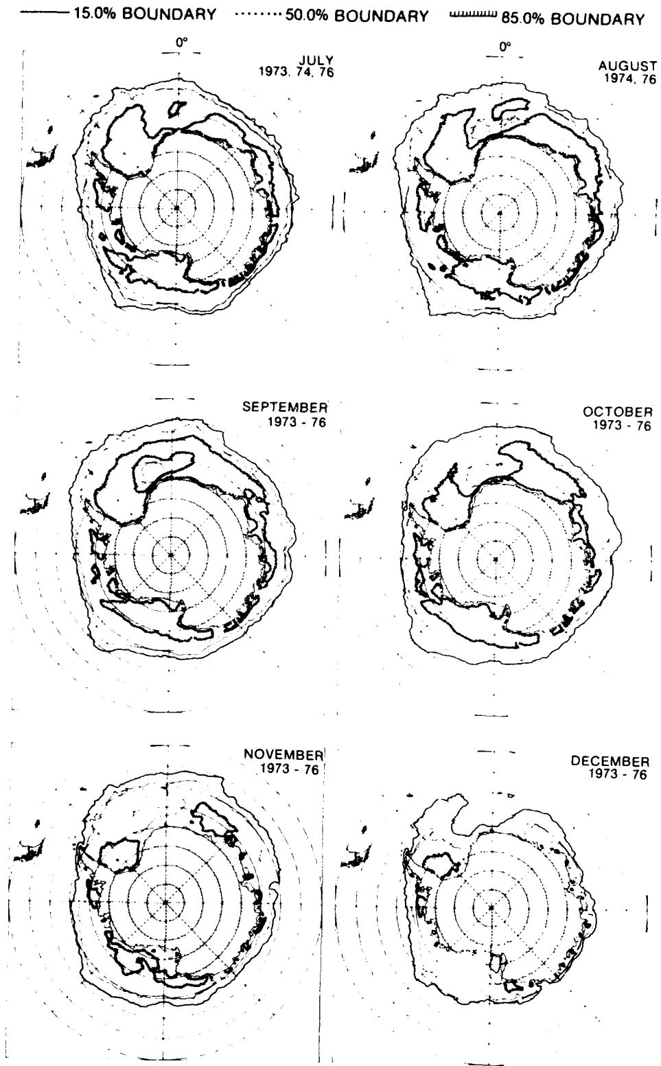
Figure B-11b. Mean monthly ice concentration contours for July through December, averaged for the years indicated.
