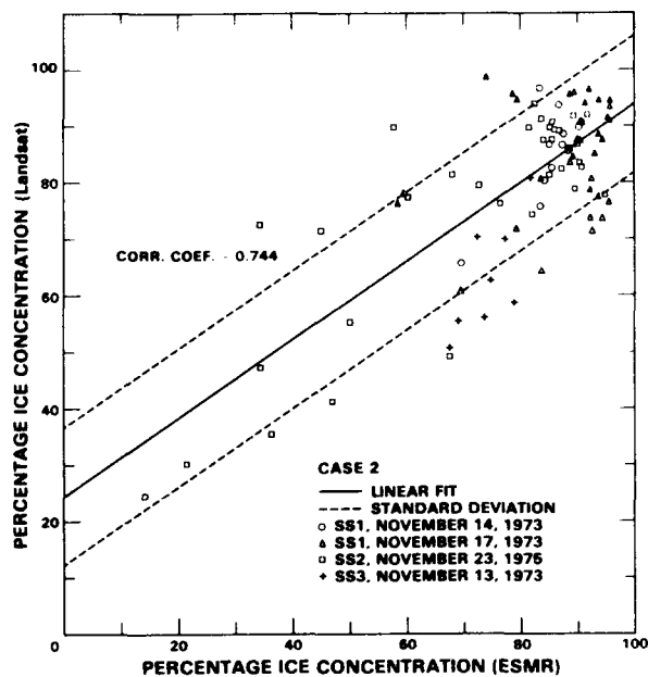
Figure 3-26. Comparison of sea ice concentrations derived from ESMR data with those from Landsat data (from Comiso and Zwally, 1982).
