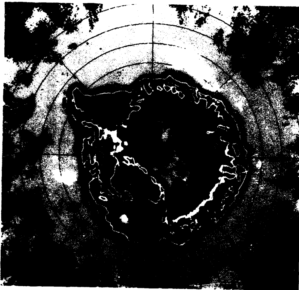
Figure 3-7b. Mean monthly brightness temperatures for April 1975 and 1976.
