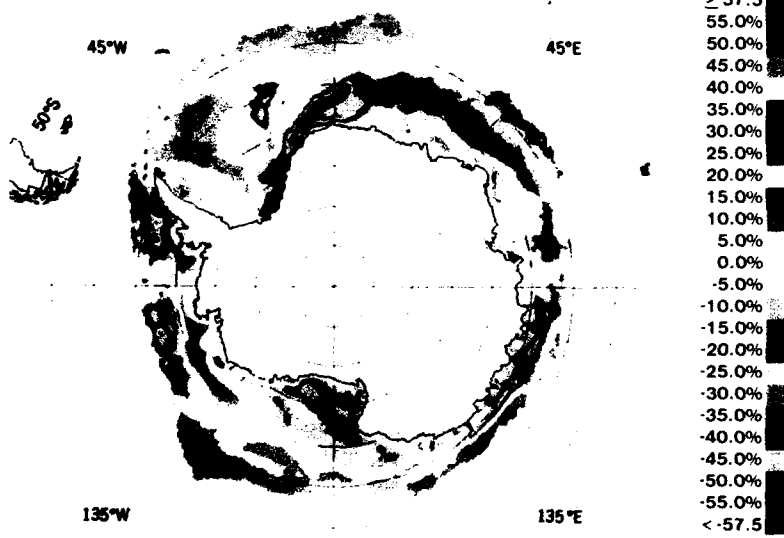
Figure 5-40. Change in annual mean sea ice concentrations from 1973 to 1974, from 1974 to 1975, and from 1975 to 1976.
