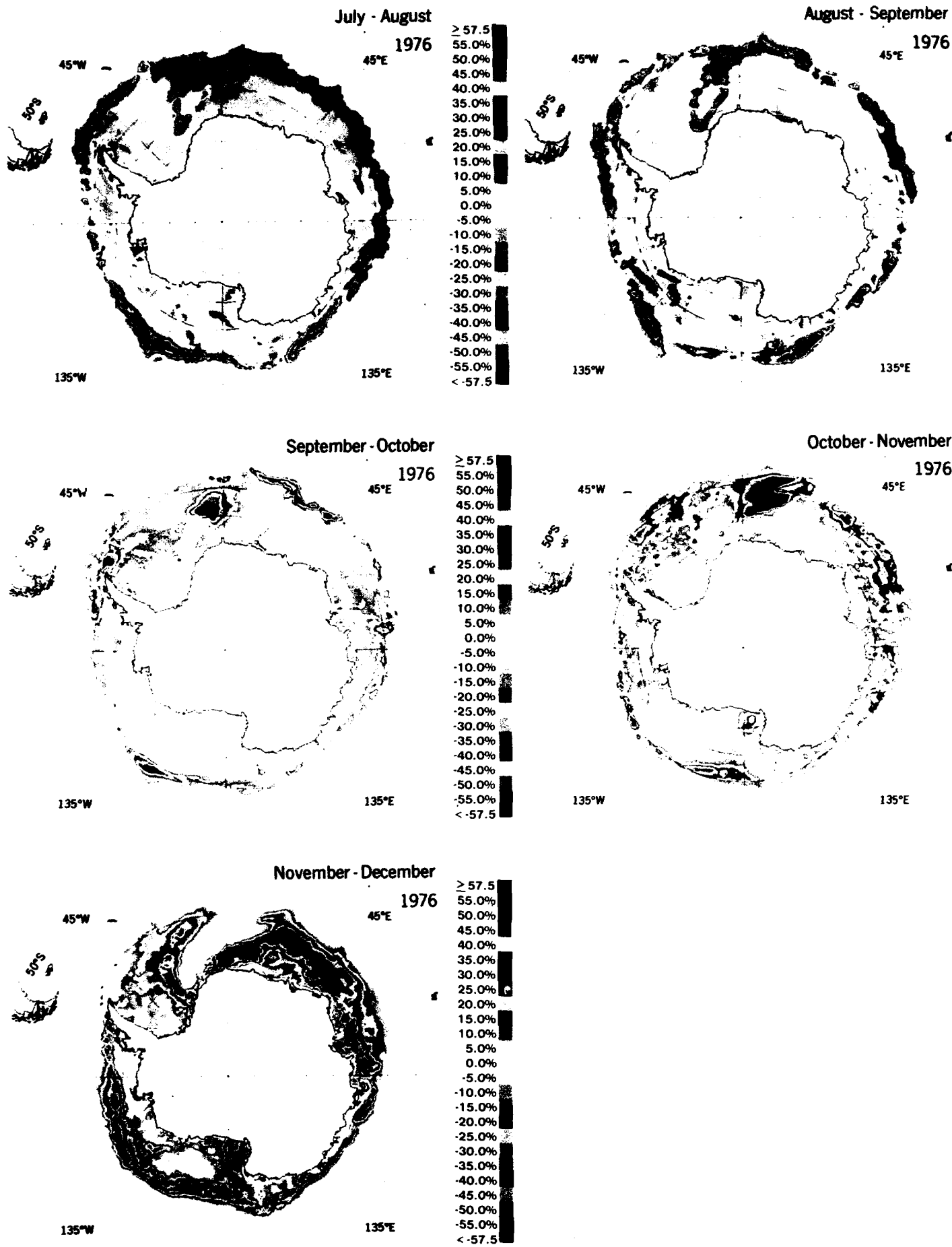
Figure 5-26b. Sea ice concentration monthly change maps for July-August 1976 through November-December 1976.
