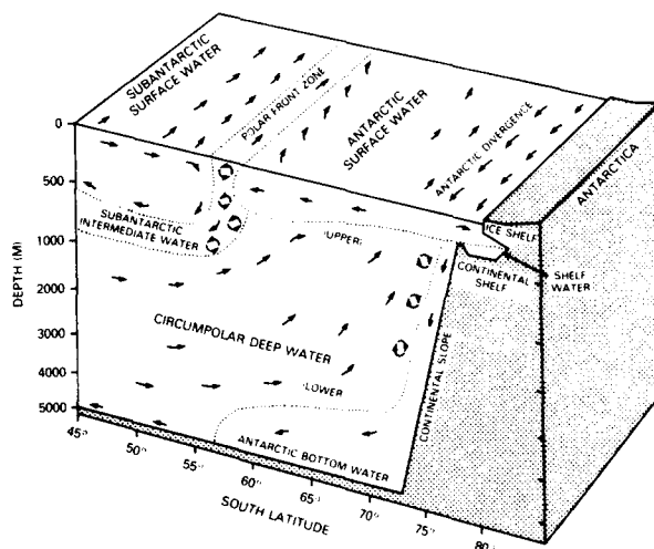
Figure 2-4. Schematic representation of water-mass types and motions (from Gordon and Goldberg, 1970).
