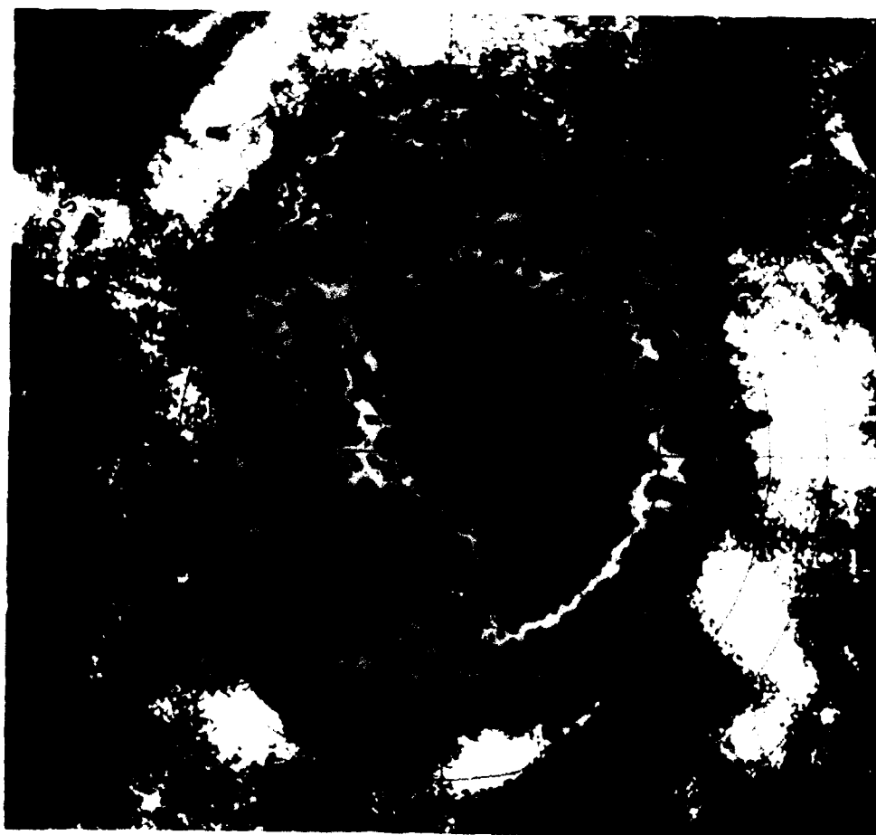
Figure 3-3a. Three-day average of brightness temperatures for December 2 through 4, 1973, and November 30 through December 2, 1974.
