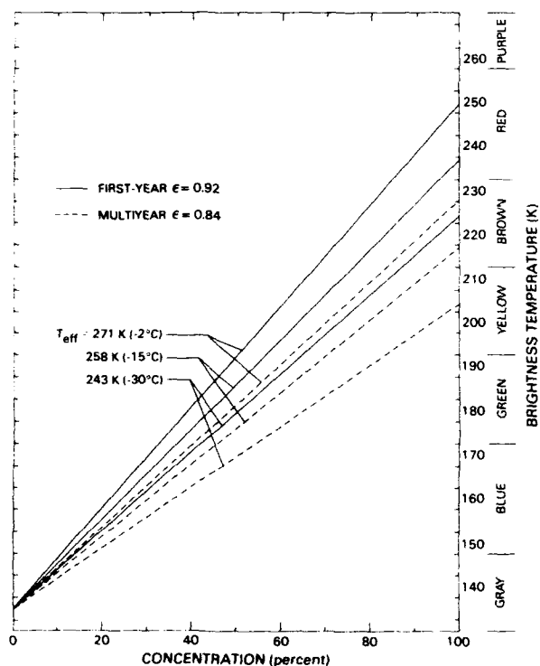
Figure 3-23. Linear relationship between sea ice concentration and microwave brightness temperature (see equation 3-5) for two values of emissivity and several values of the effective physical temperature of the ice radiating layer.
