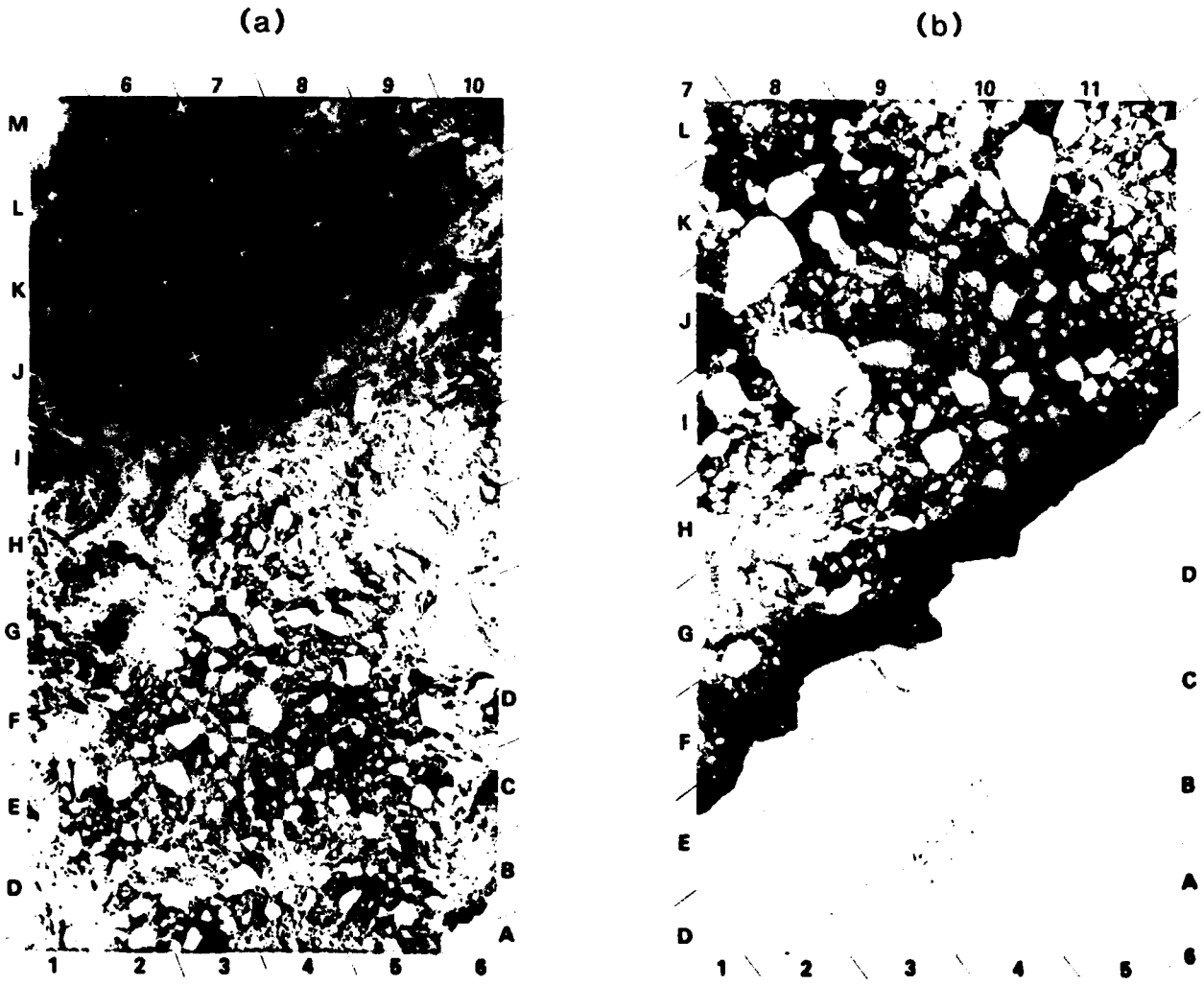
Figure 3-25. Landsat multispectral scanner images at near-infrared (1.1 microns) wavelengths: (a) image for November 23, 1975, centered at 68^{\circ}1'S , 4^{\circ}49'W and (b) image for November 13, 1973, centered at 69^{\circ}2'S , 9^{\circ}16'E .
