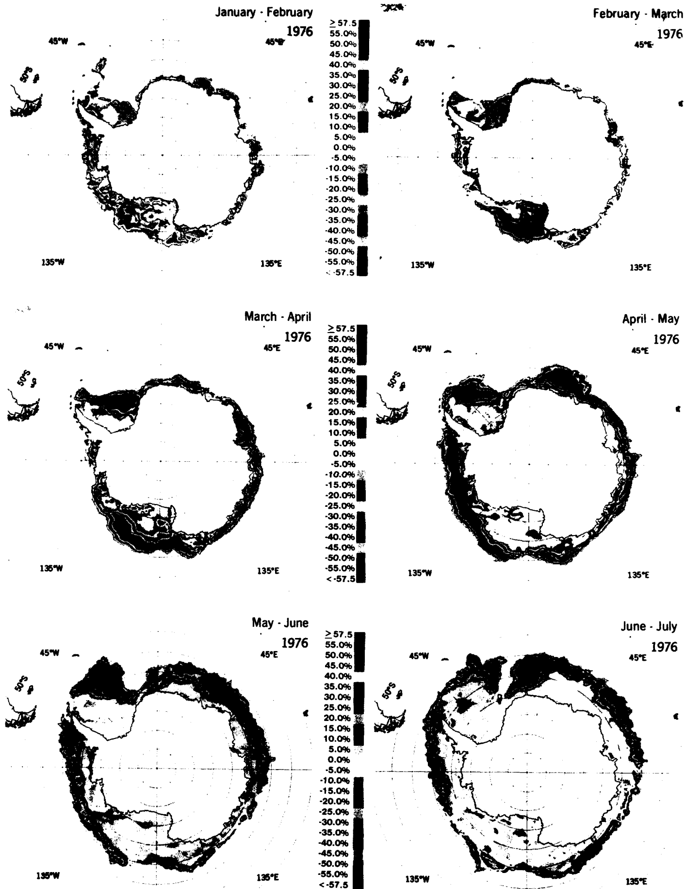
Figure 5-26a. Sea ice concentration monthly change maps for January-February 1976 through June-July 1976.
