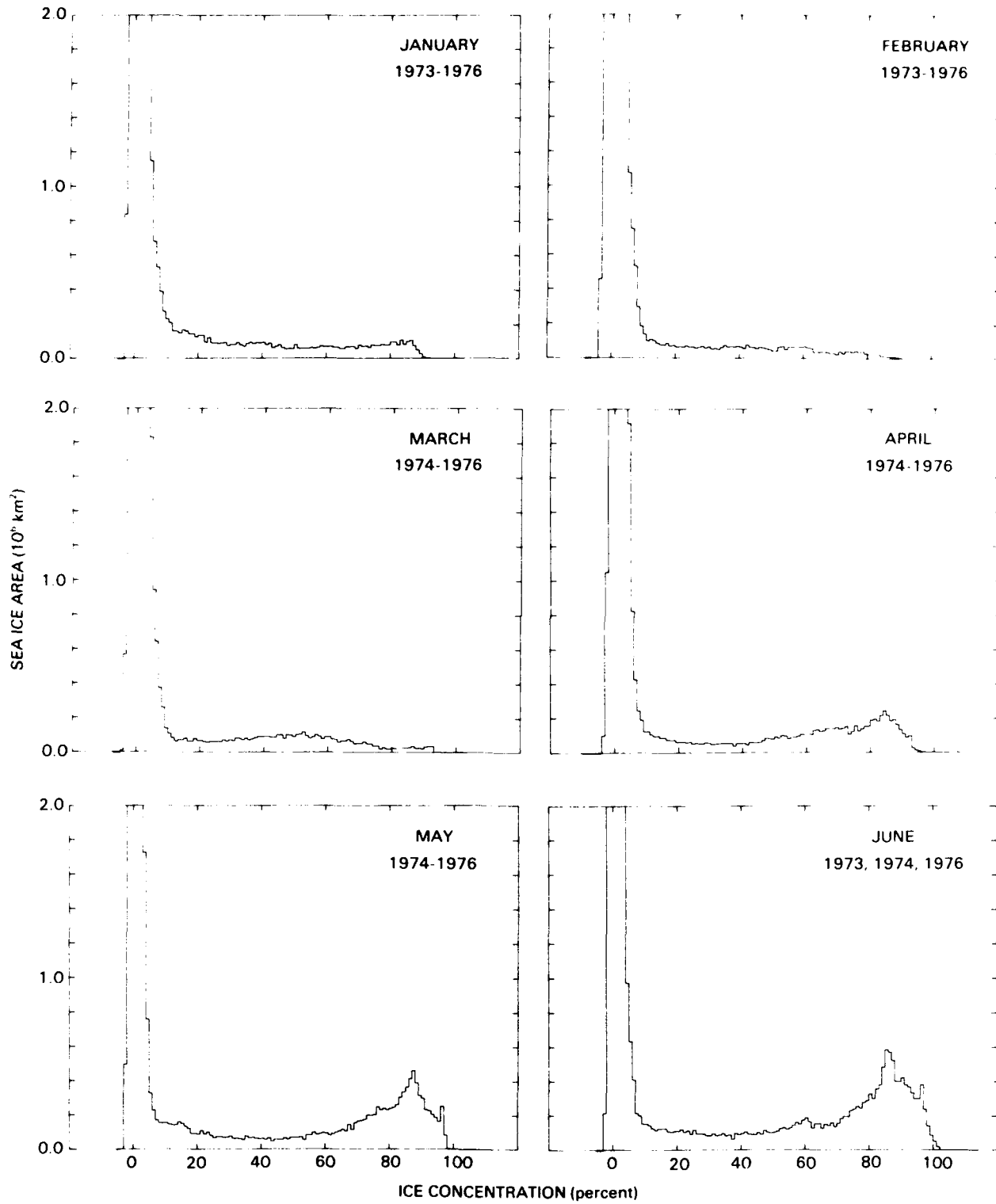
Figure C-1a. Areal distribution of percentage ice concentration in all sectors from January to June (1973-1976).
