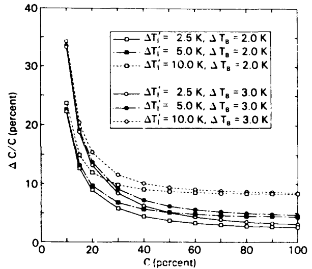
Figure 3-28. Uncertainty in ice concentration derived from ESMR data as a function of ice concentration, presented for several errors in brightness temperature ( \Delta T_B = 2.0 and 3.0 K) and for several errors in estimated snow/ice interface temperature ( \Delta T_1' = 2.5, 5.0, and 10 K).
