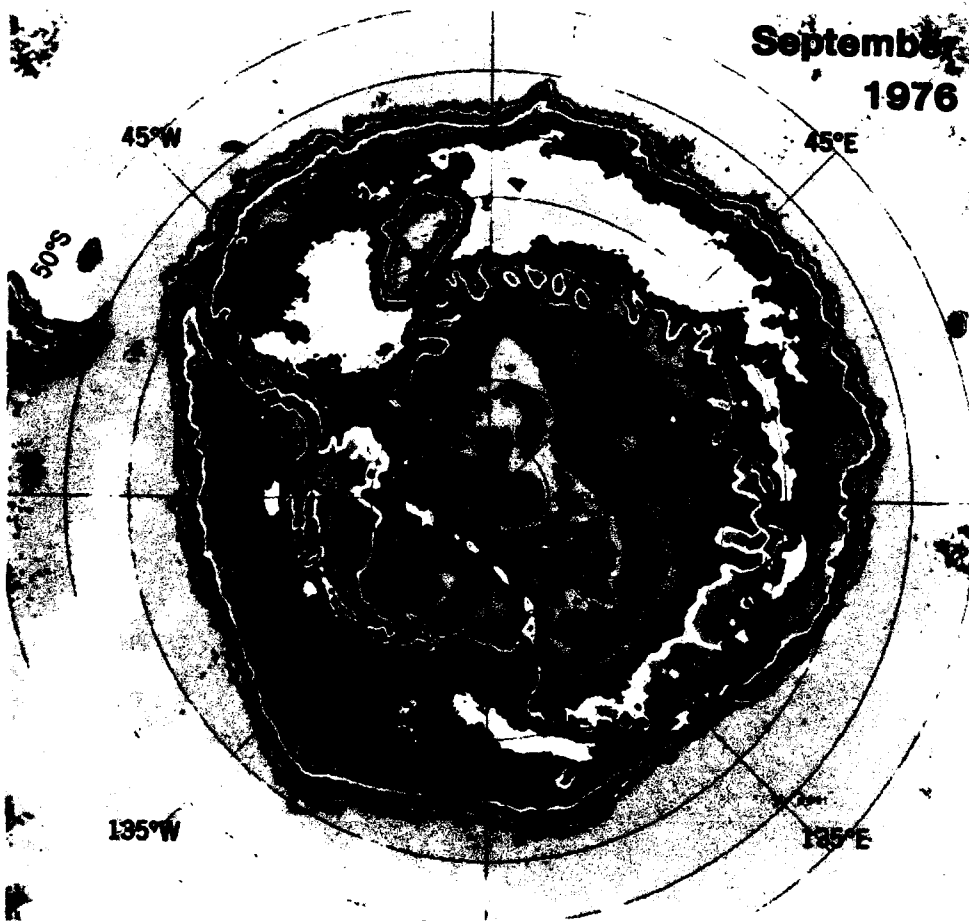
Figure 3-12b. Mean monthly brightness temperatures for September 1975 and 1976.
