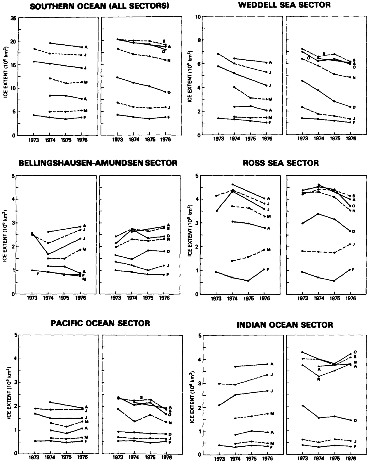
Figure 5-35. Year-to-year changes in sea ice extent for each month, for the total southern ocean and each sector.
