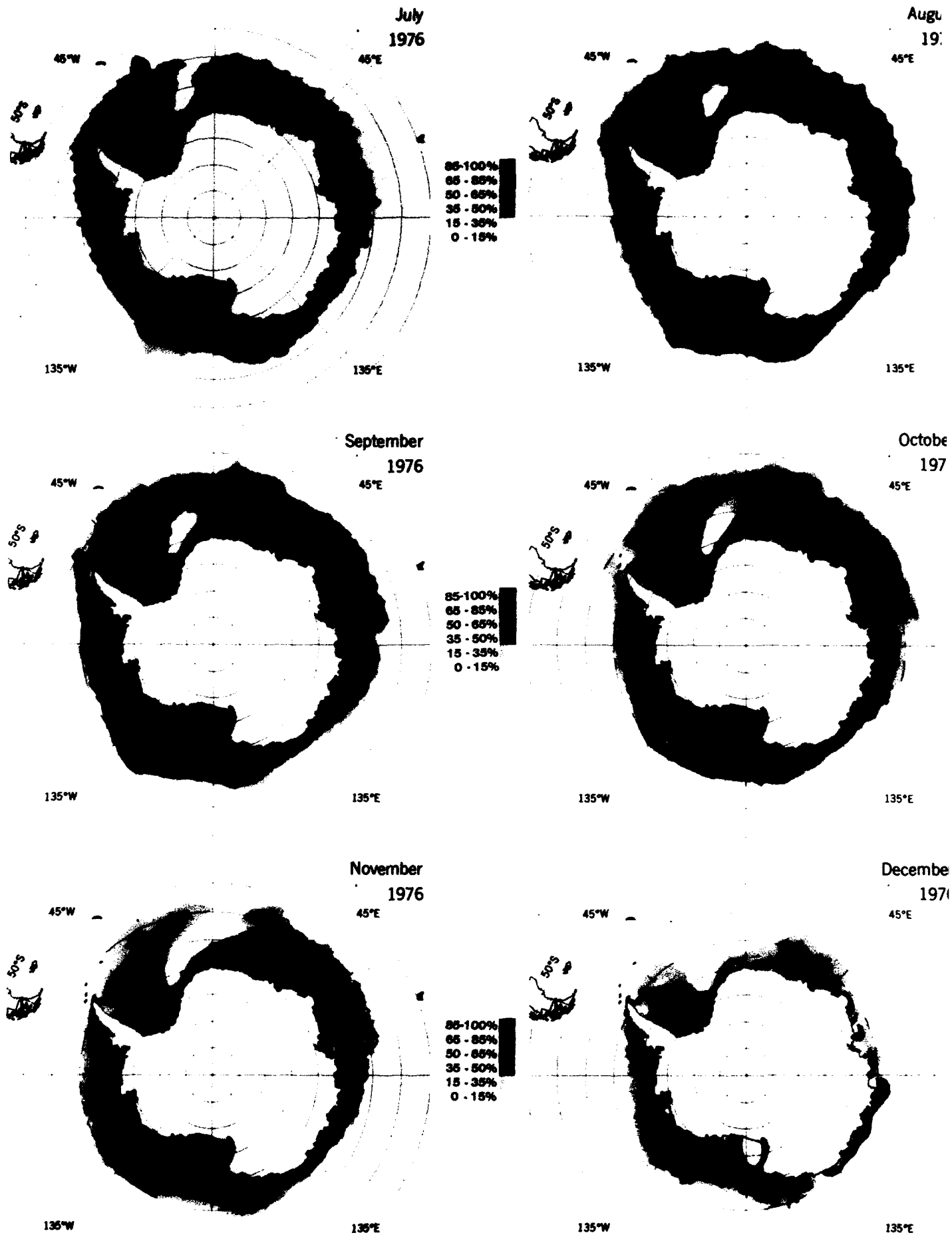
Figure B-4b. Mean monthly ice concentrations for July through December 1976.
