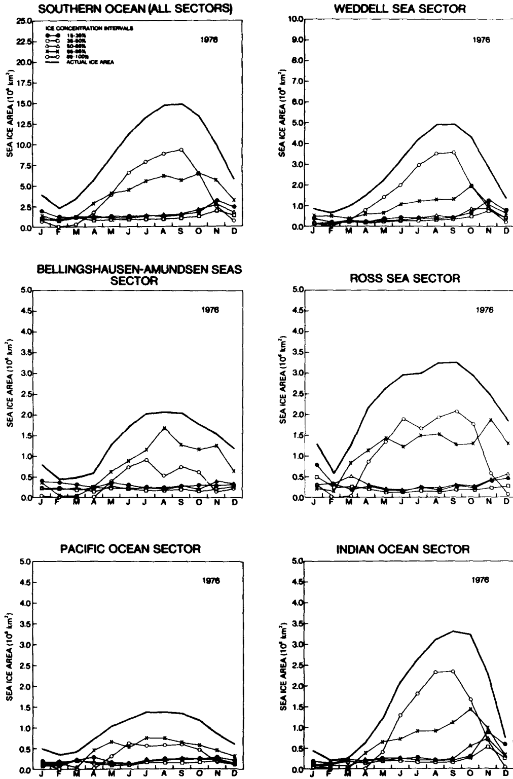
Figure 5-22. Yearly cycle (for 1976) of the ocean area covered by sea ice within ice concentration intervals 15 to 35, 35 to 50, 50 to 65, 65 to 85, 85 to 100 percent and yearly cycle of the actual ice area, for the total southern ocean and for each sector.
