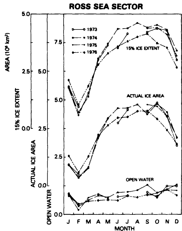
Figure 5-30. Interannual variation of the yearly cycle of the 15-percent extent, the actual ice area, and the open water within the ice pack for the Ross Sea sector.
