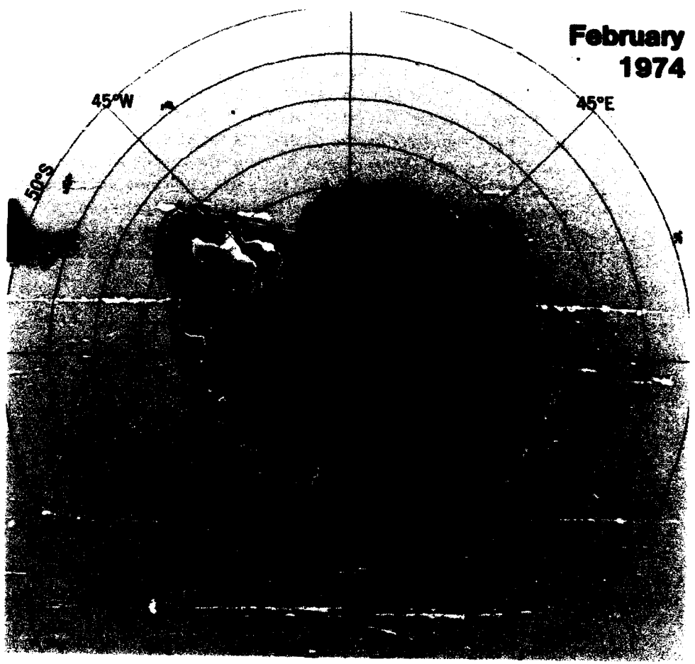
Figure 5-2a. Mean monthly sea ice concentrations for February 1973 and 1974.
