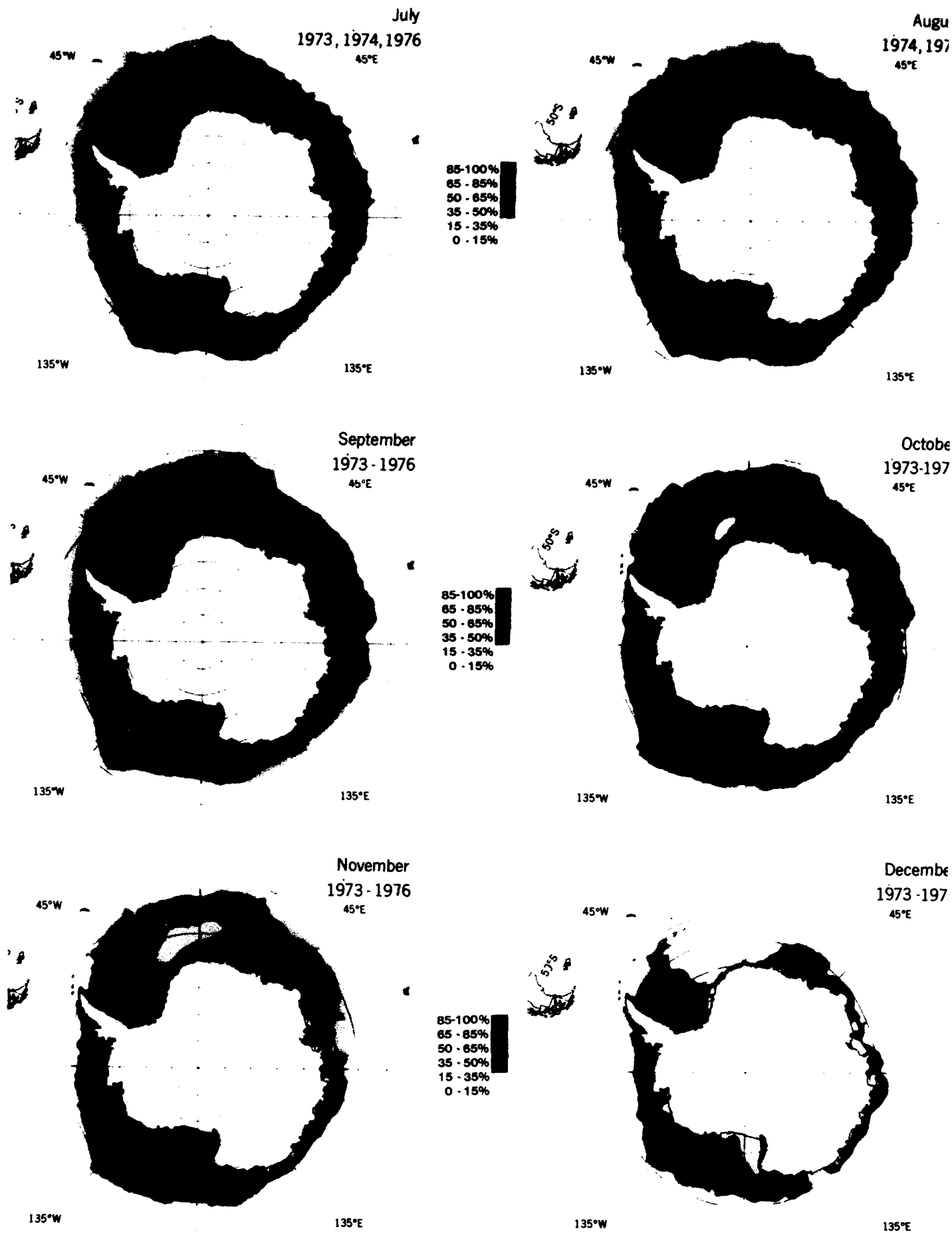
Figure B-5b. Mean monthly ice concentrations for July through December, averaged for the years indicated.
