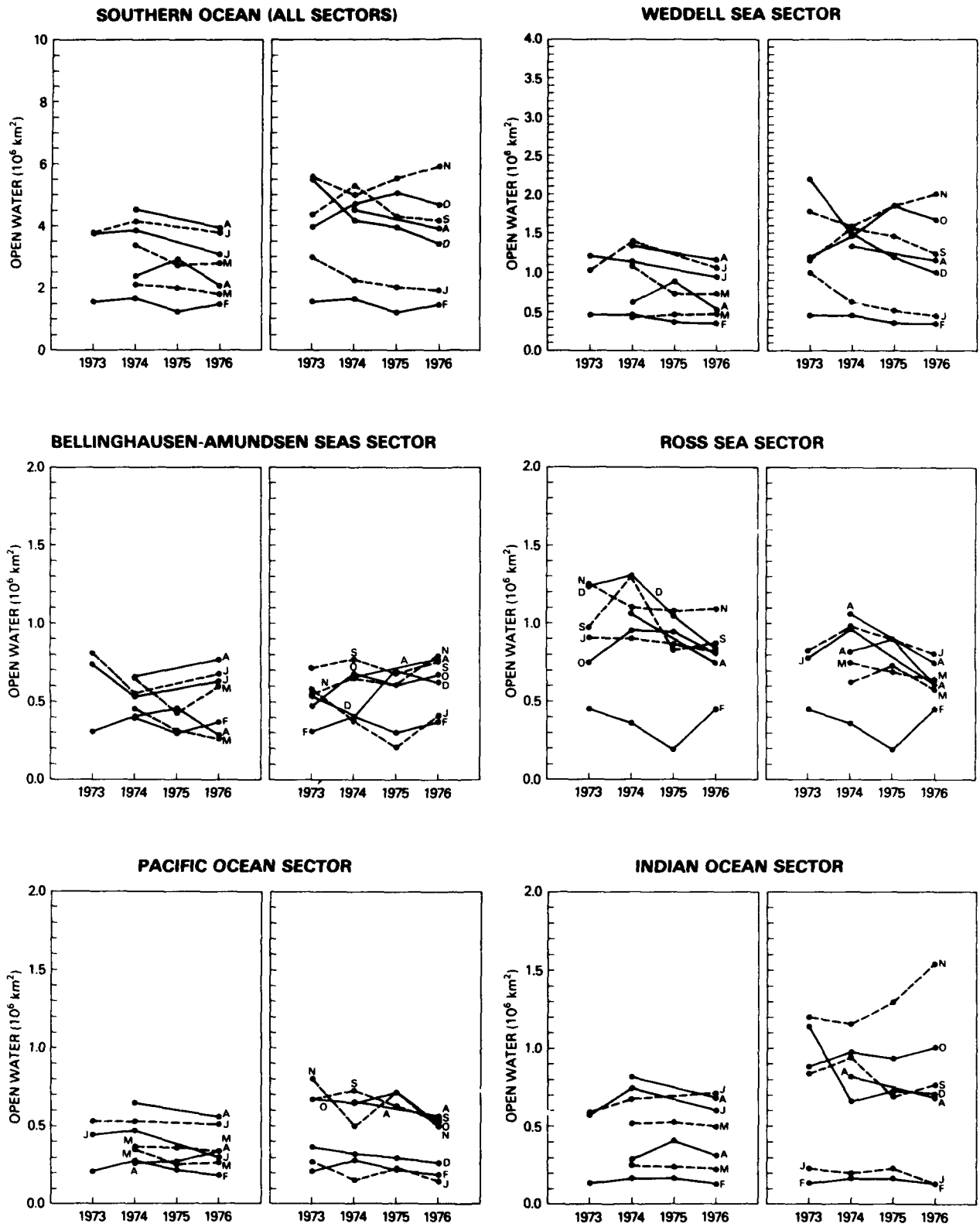
Figure 5-37. Year-to-year changes in open water within the ice pack, for the total southern ocean and each sector.
