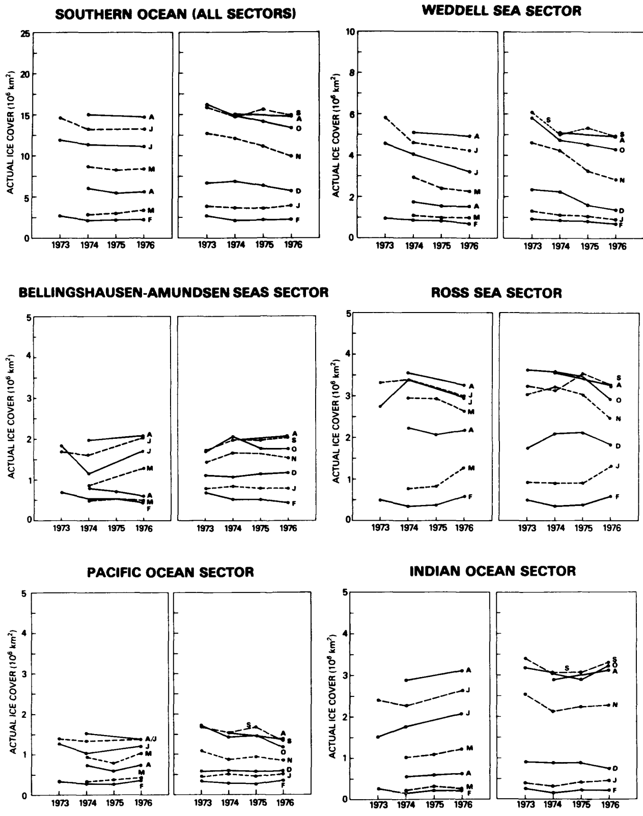
Figure 5-36. Year-to-year changes in actual ice area for each month, for the total southern ocean and each sector.
